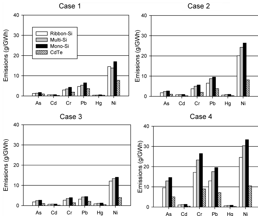
FIGURE 4. Life-cycle atmospheric heavy-metal emissions for PV systems (normalized for Southern European average insolation of 1700 kWh/m 2 /yr, performance ratio of 0.8, and lifetime of 30 yrs). Each PV system is assumed to include a ground-mounted BOS as described by Mason et al. (18). The four types of PV modules and corresponding efficiencies are ribbon-Si 11.5%, multi-crystalline Si 13.2%, monocrystalline 14%, and CdTe 9%.
